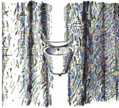
Fig. 372.*—Hugues' collar and pot.
